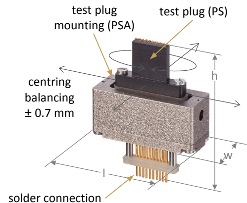
Connector contacting (STK) STK-1,00-M-010-JST (Part no. 49911)
